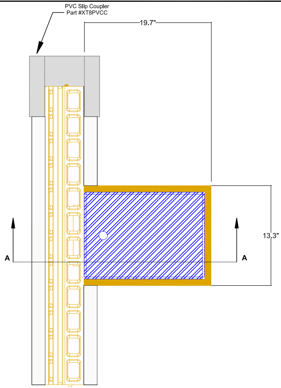
PLAN VIEW
