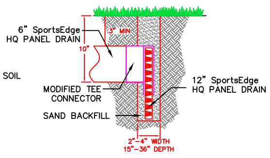
PERIMETER DRAIN DETAIL
