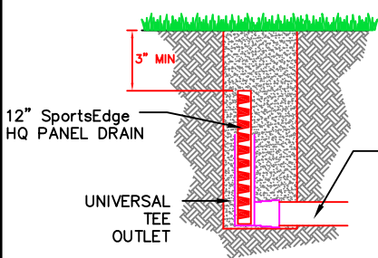
PERIMETER DRAIN DETAIL
