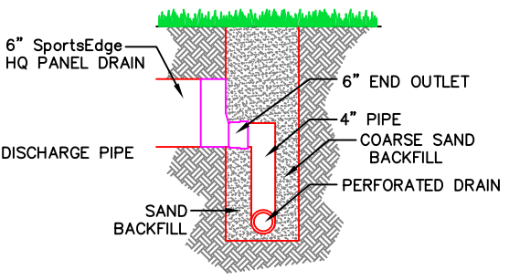
PERIMETER DRAIN DETAIL PIPE OPTION
