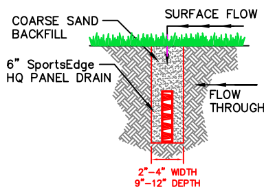
FIELD DRAIN DETAIL
