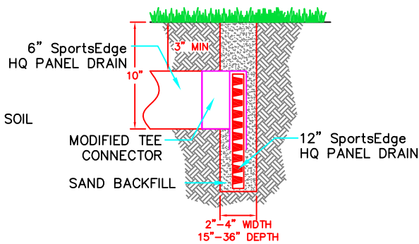
PERIMETER DRAIN DETAIL
