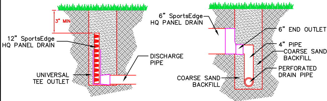
PERIMETER DRAIN DETAIL PIPE OPTION
