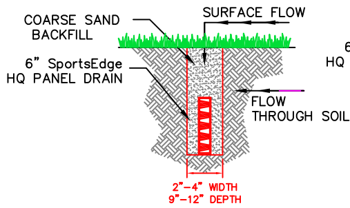
FIELD DRAIN DETAIL
