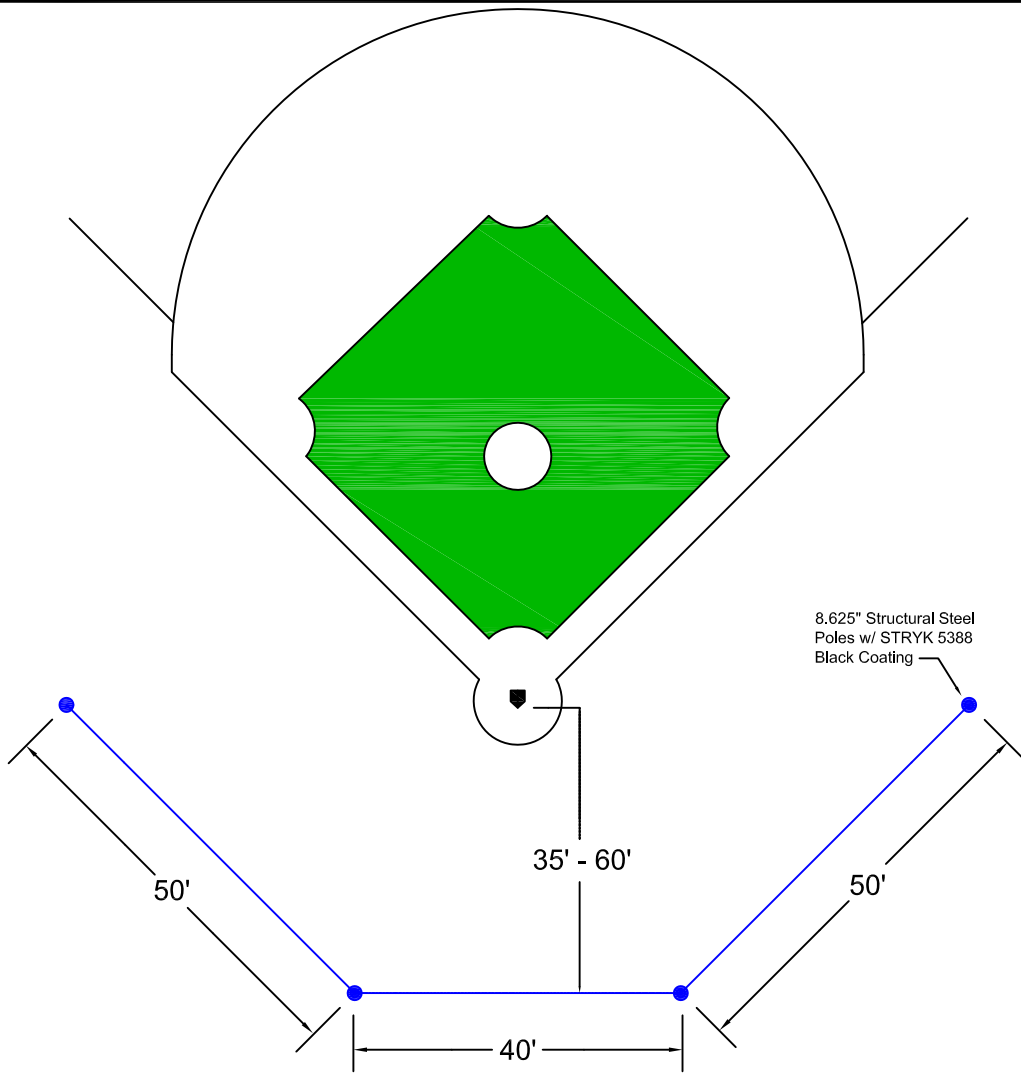
PLAN - POLE LAYOUT PREMIER BASEBALL BACKSTOP
