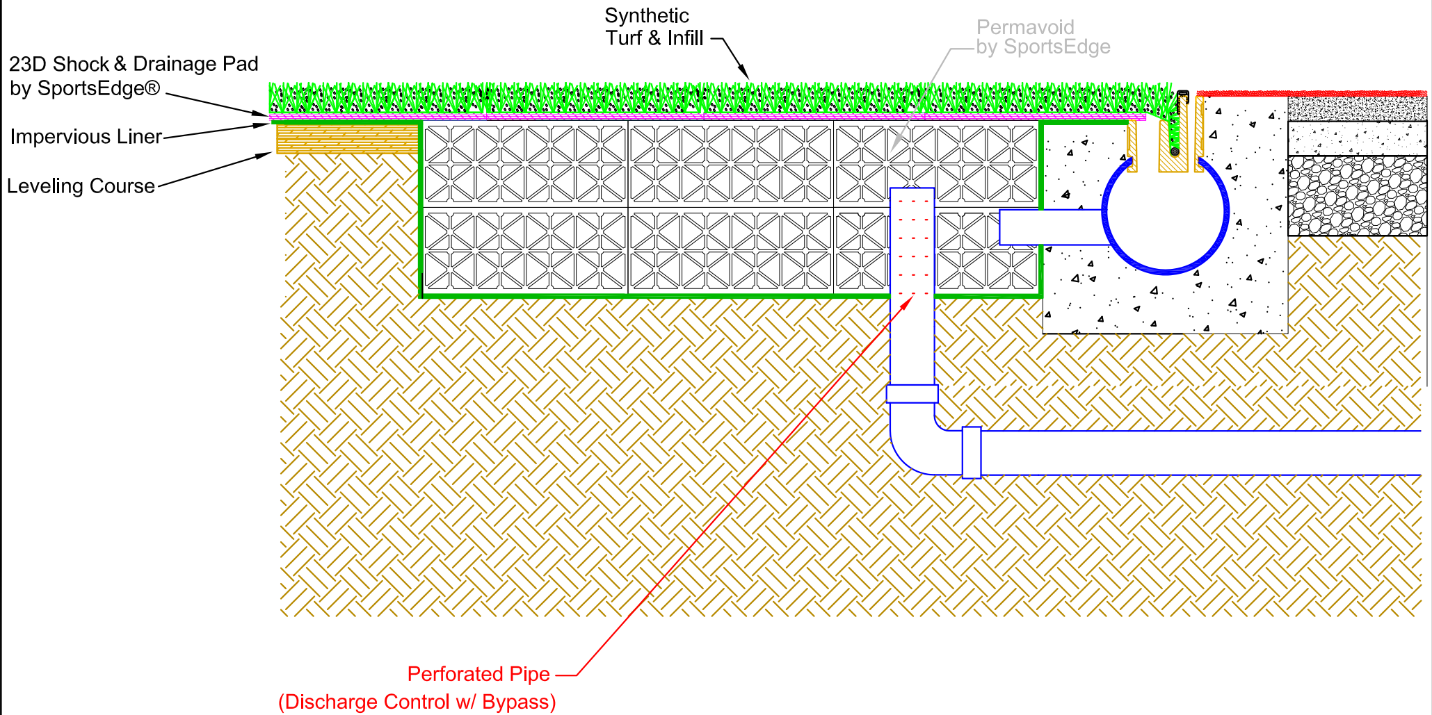
Plan View- SportsEdge Terminator Drain System w/ Permavoid Water Control System
