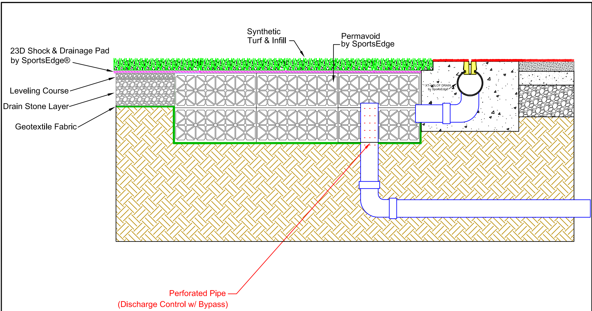
Plan View- SportsEdge XT-4 Surface Drain System w/ Permavoid Water Control System
