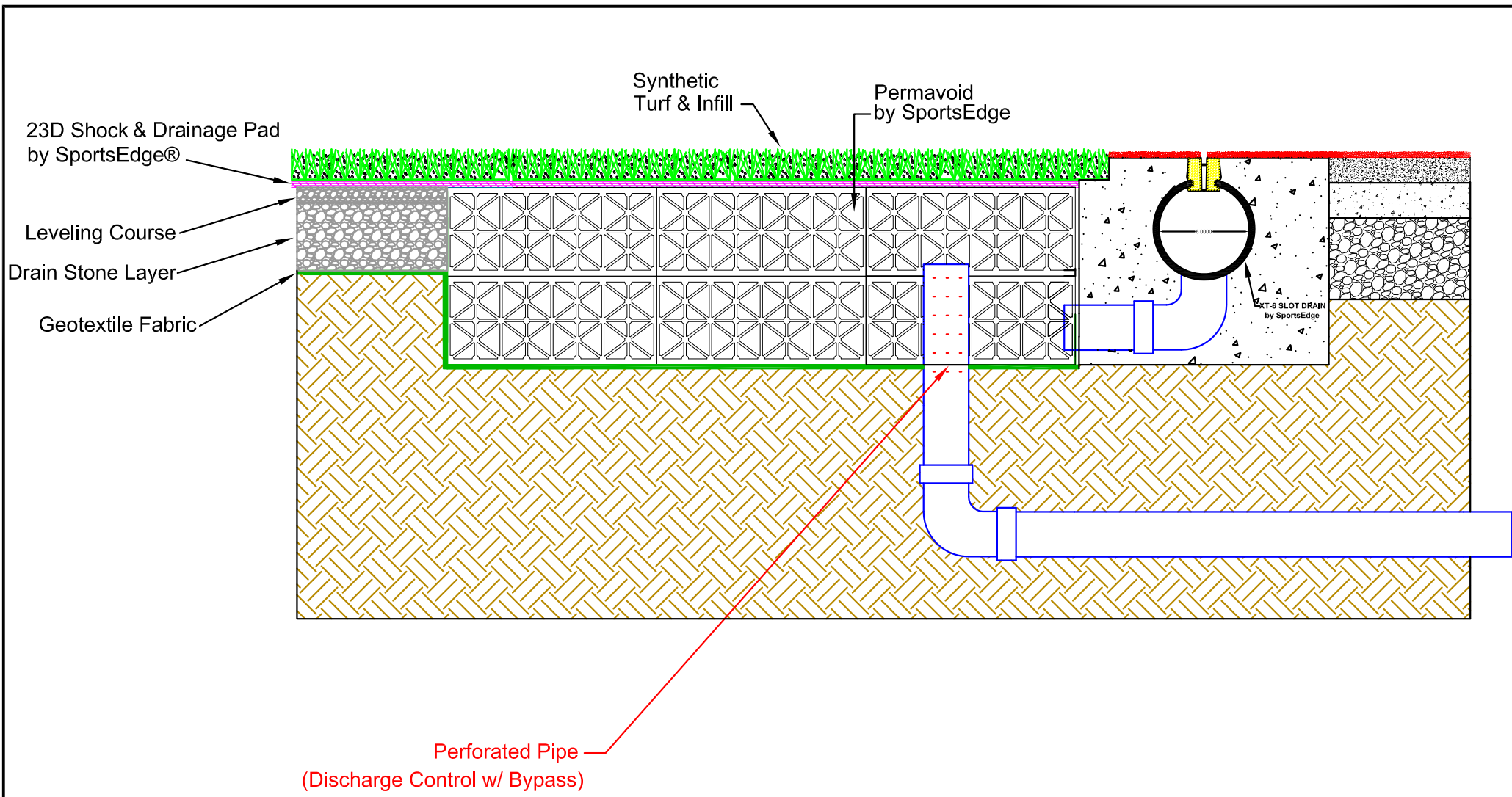
Plan View- SportsEdge XT-6 Surface Drain System w/ 23D Shock/Drain Pad and Permavoid Water Control System
